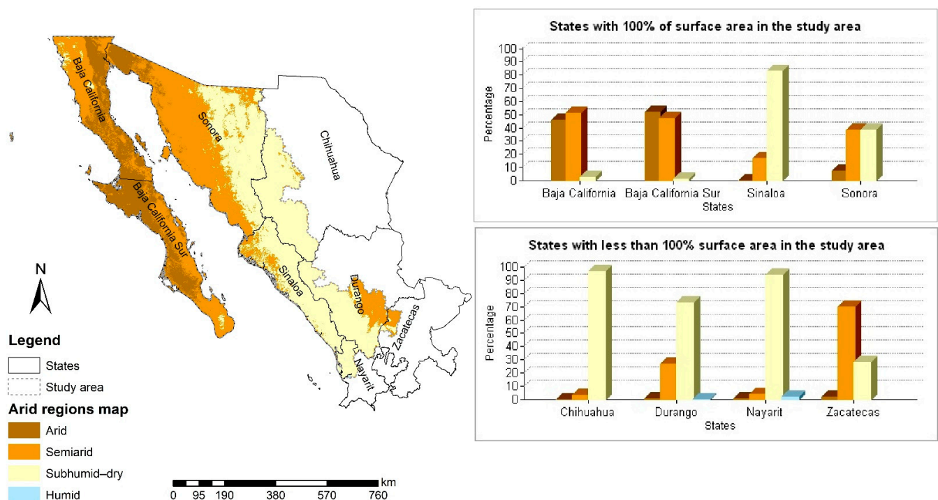
Figure 8. Map of arid zones and graphs representing the level of aridity by state.
